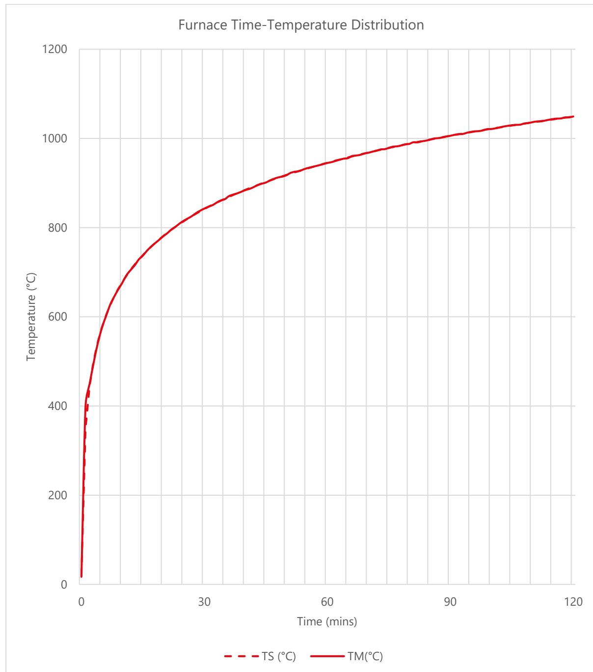
Figure 1 Time-Temperature Distribution
