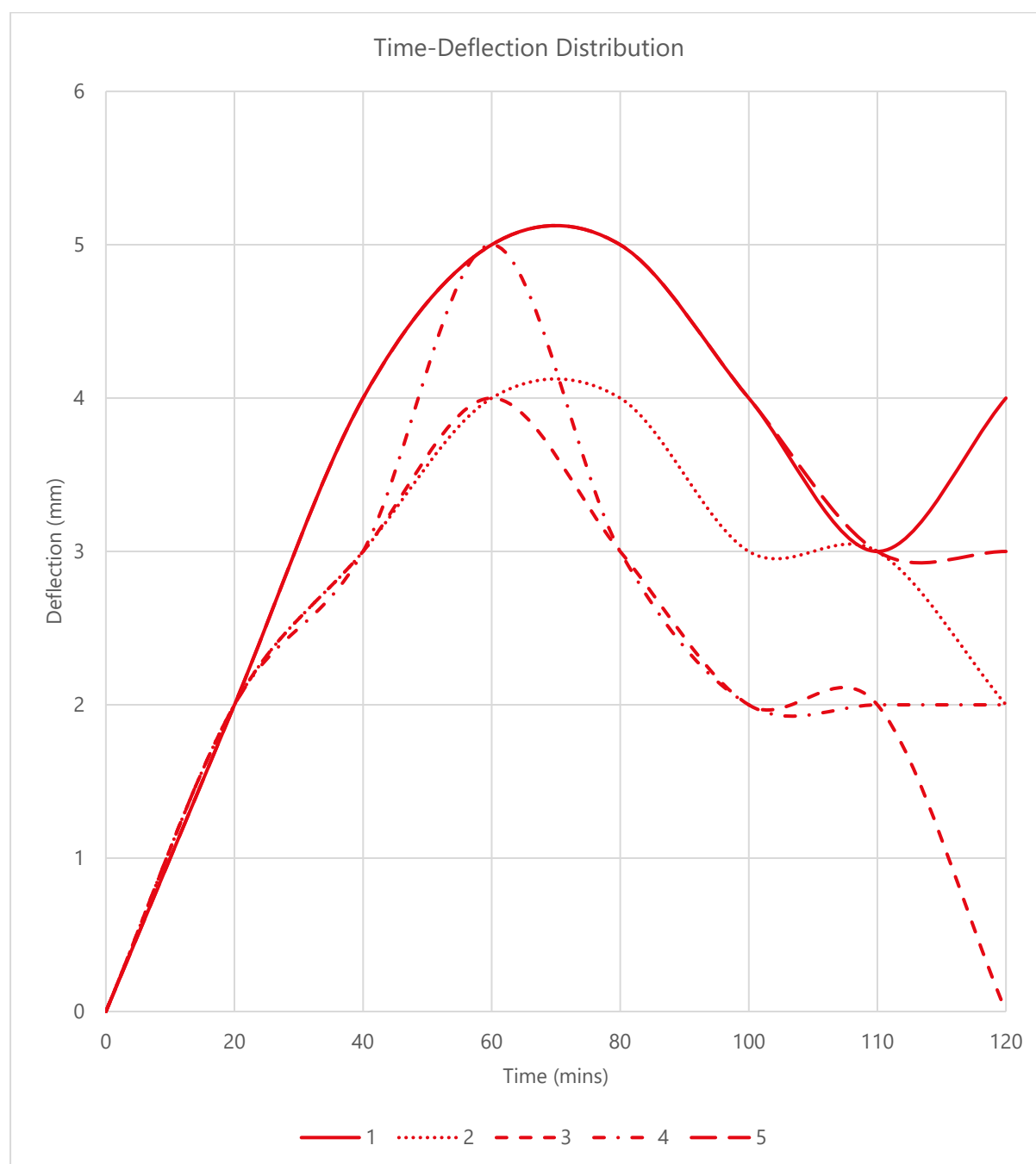
Figure 6 Time-Deflection Distribution
